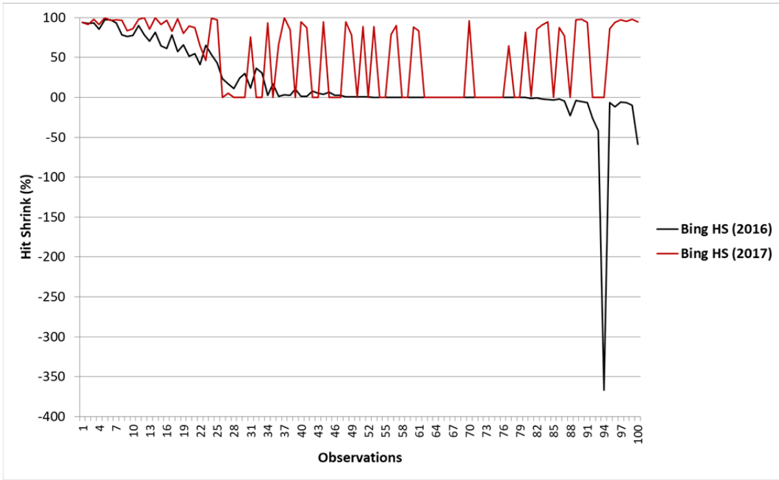
Fig.7. Variation of the hit shrink rate between 2016 and 2017 in Bing.
