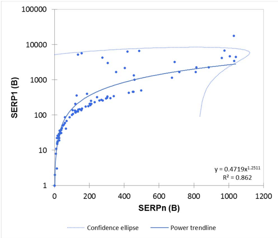
Fig.5. Power trendline between SERP_1 (B) and SERP_n (B).
