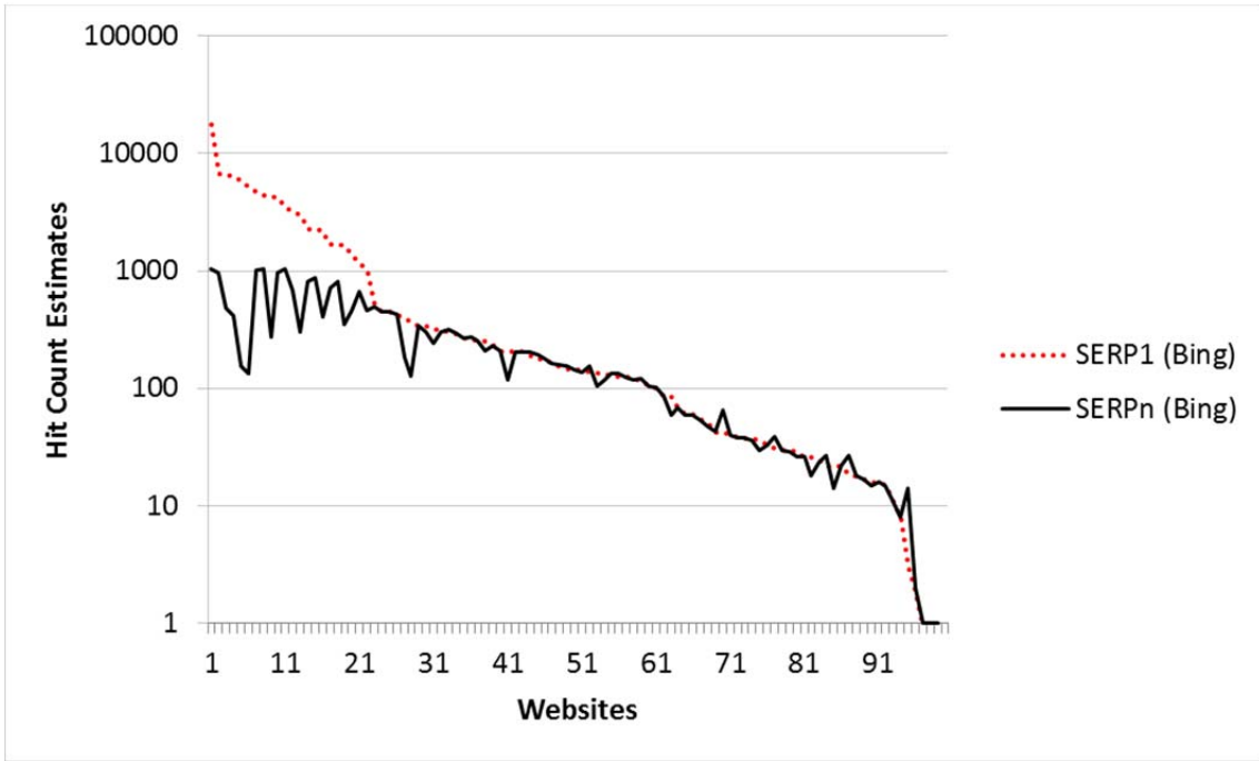
Fig.3. Web size distribution for rare disease associations according to SERP (Bing).
